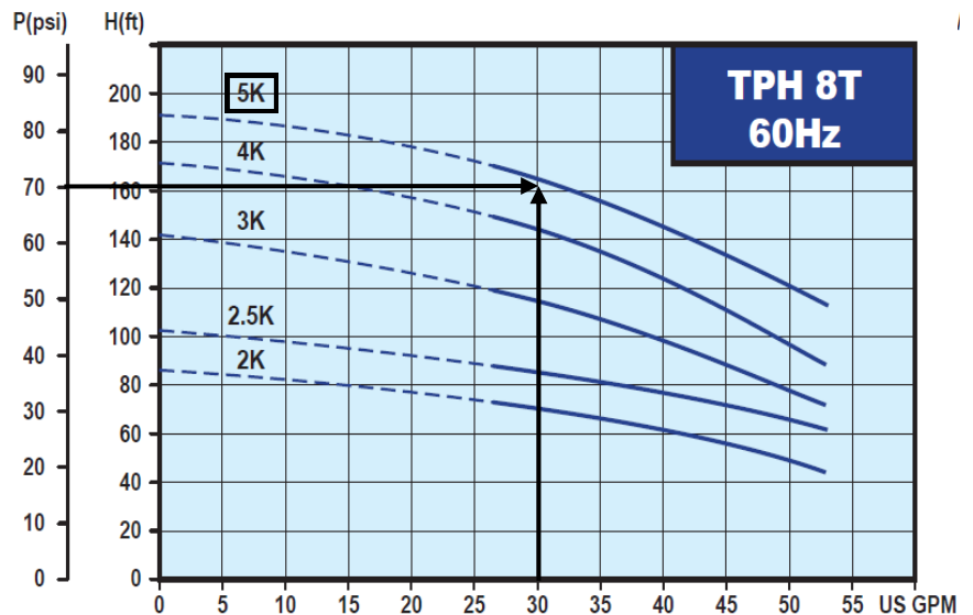
Pump performance curve
