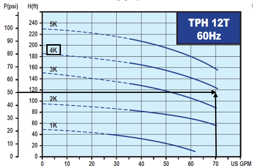
Pump performance curve
