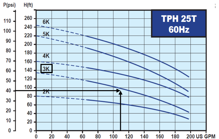
Performance curve for each pump
